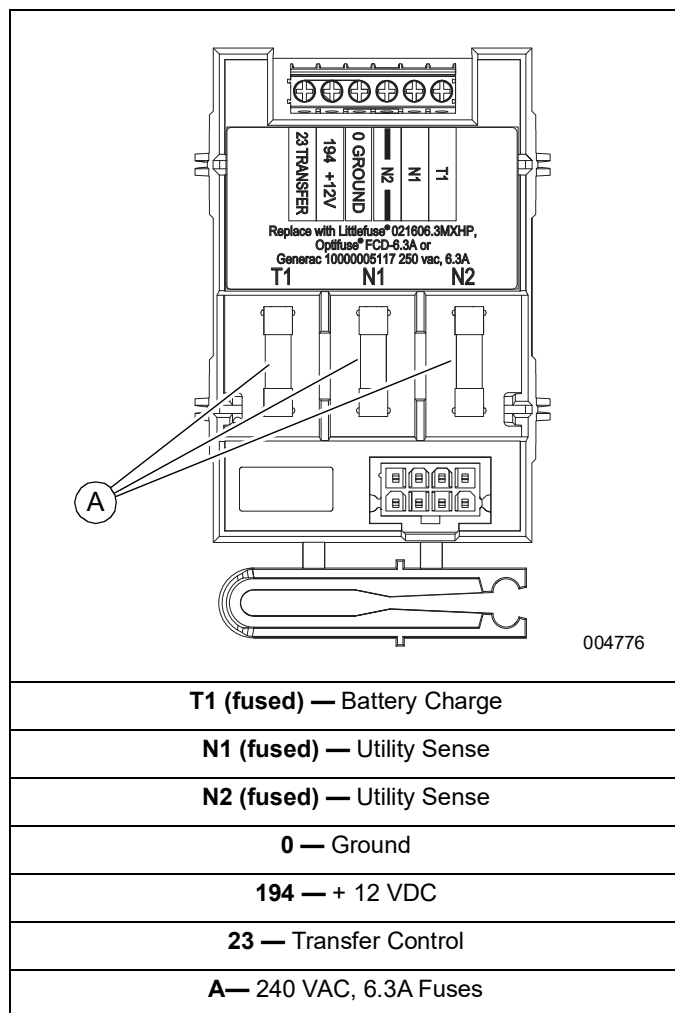
Figure 3-2. Typical Connections
