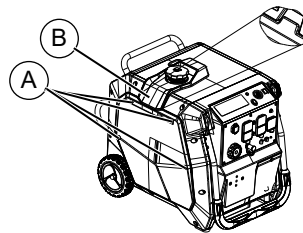
Figure 2-10. Access Door
