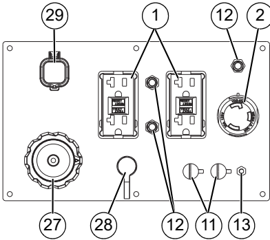
Figura 2-3. Panel de control frontal
